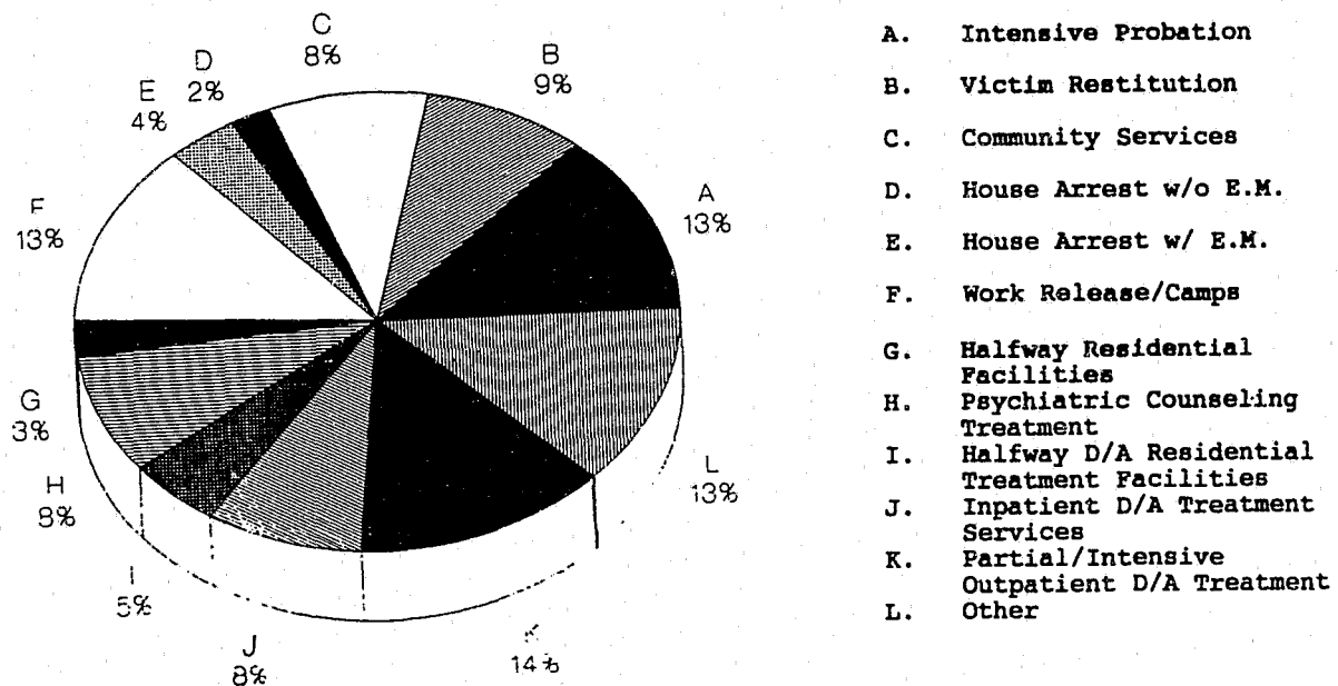
FIGURE 2 PROGRAM TYPES
