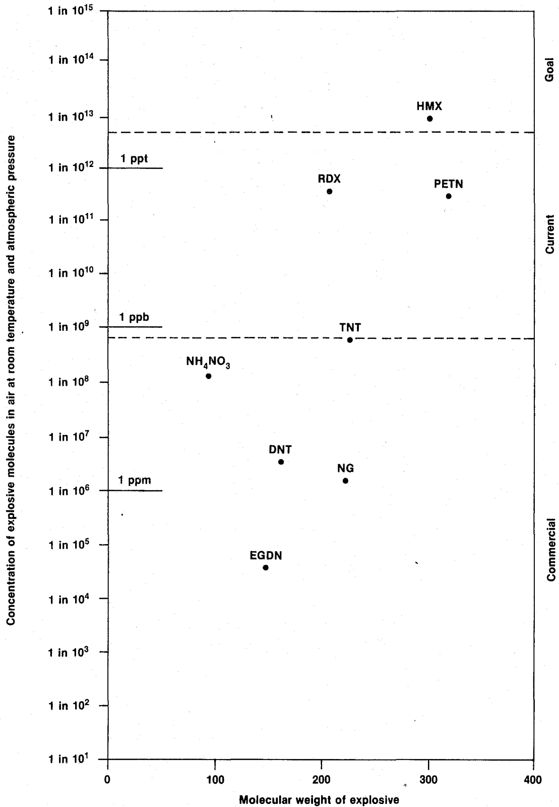
Figure 4-5—Relative Volatilities of Some Common Explosives
