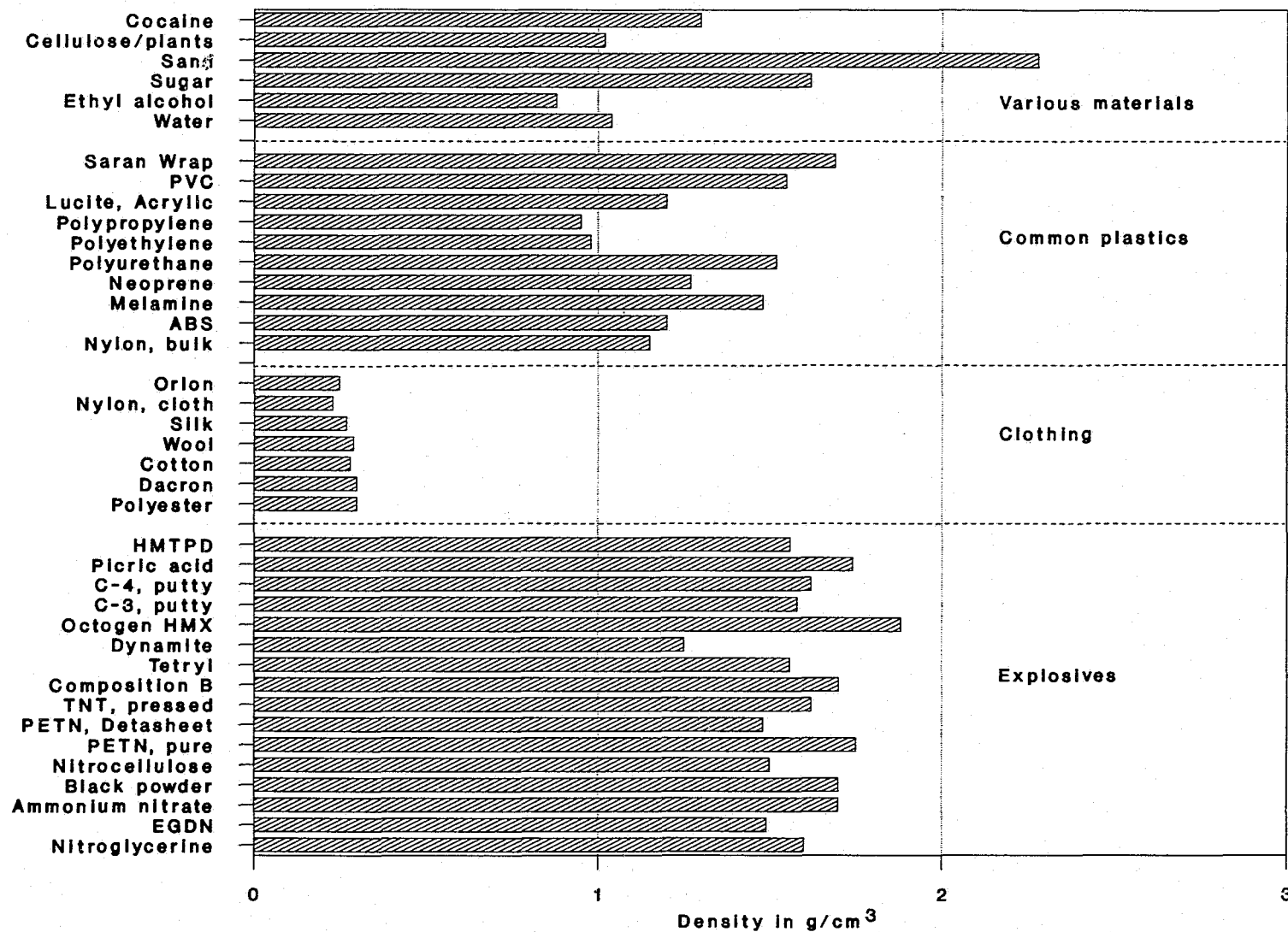
Figure 4-1—Densities of Various Materials
