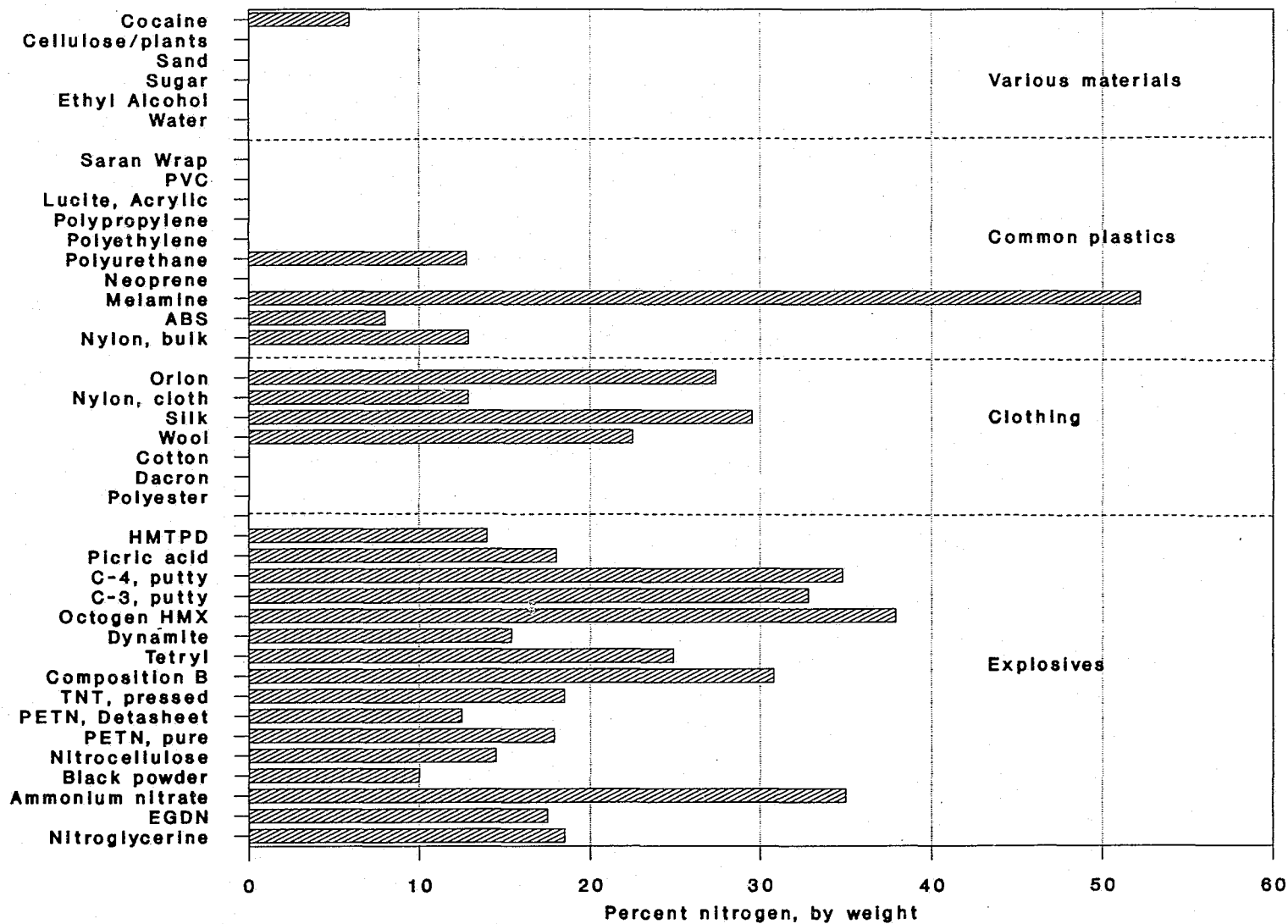
Figure 4-2—Nitrogen Percentage of Various Materials
