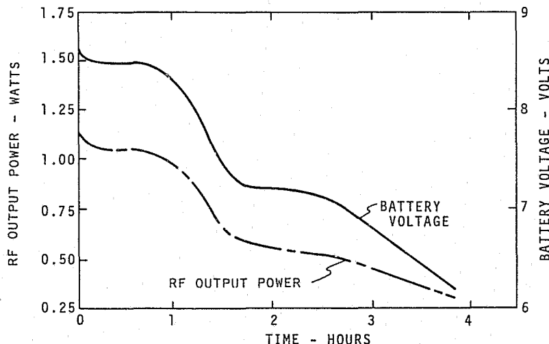
FIGURE 7. Decay of output power and battery voltage for transmitter #1.
