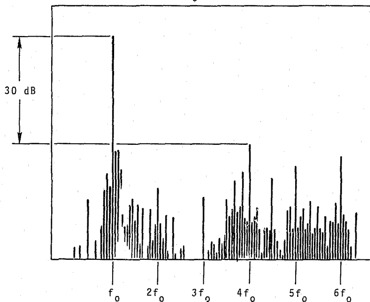
FIGURE 16. Output spectrum of transmitter #5.
