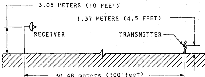
FIGURE 18. Test setup for field performance studies of body-worn transmitters.
