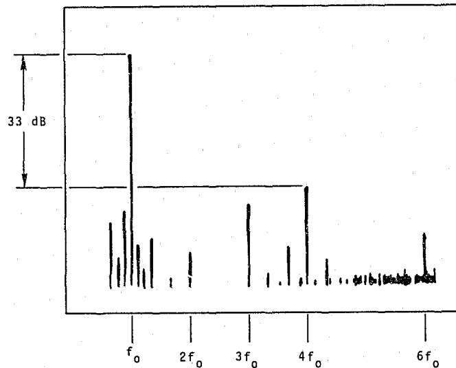
FIGURE 10. Output spectrum of transmitter #2.
