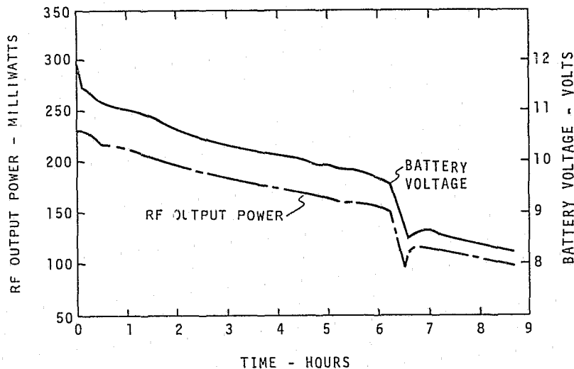
FIGURE 11. Decay of output power and battery voltage for transmitter #3.
