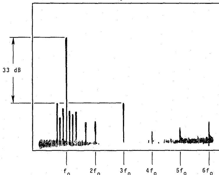
FIGURE 8. Output spectrum of transmitter #1.
