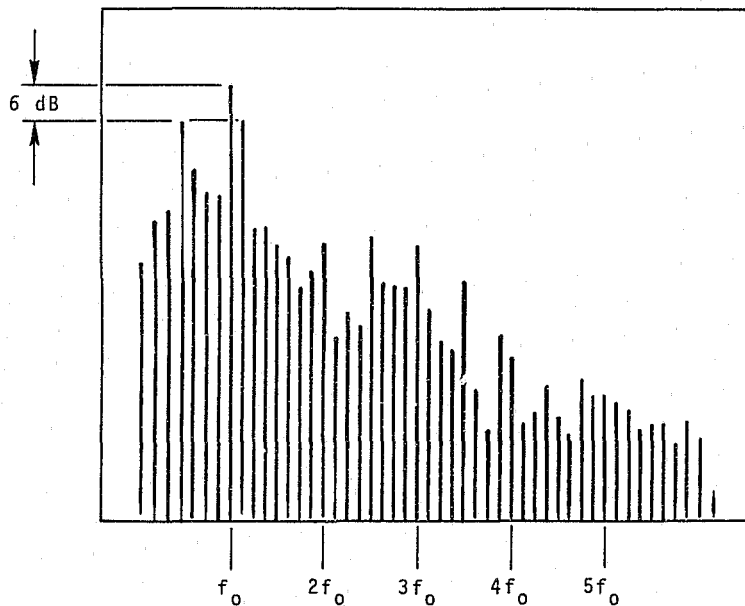
FIGURE 14. Output spectrum of transmitter #4.
