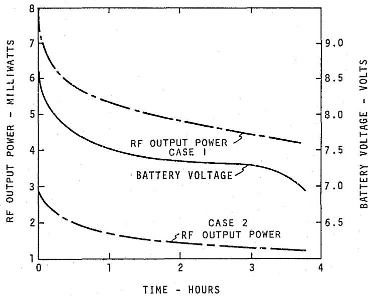
FIGURE 13. Decay of output power and battery voltage for transmitter #4.
