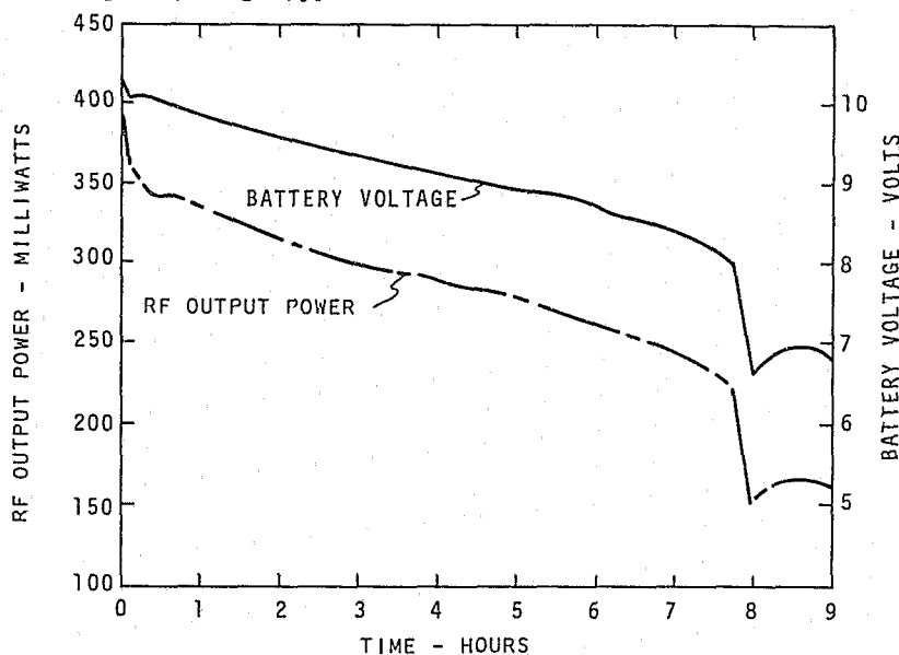
FIGURE 9. Decay of output power and battery voltage for transmitter #2.
