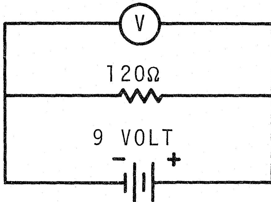
FIGURE 4. Battery test circuit.
