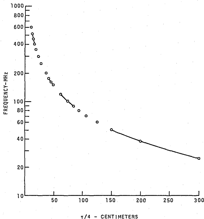
FIGURE 2. Length (in air) of quarter-wavelength antennas for the frequency range from 25 to 600 MHz.
