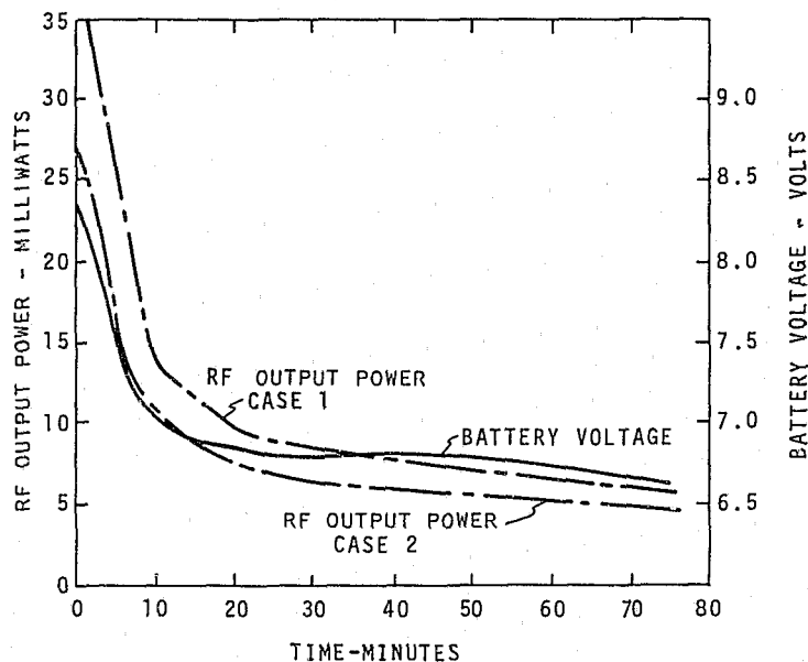
FIGURE 15. Decay of output power and battery voltage for transmitter #5.
