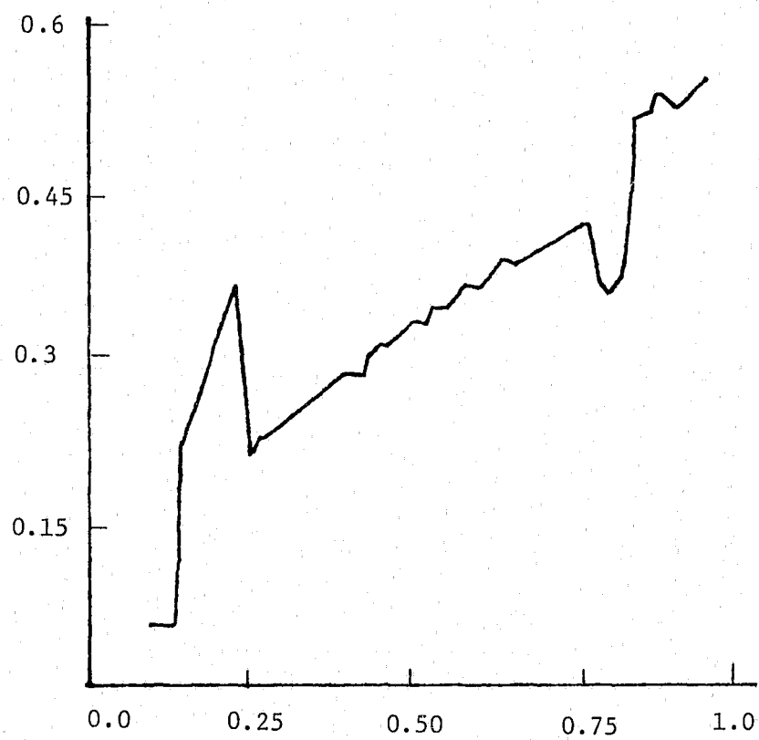
Figure 19. Q^* versus (QS)
