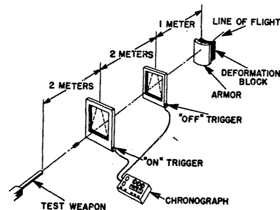
BALLISTIC DEFORMATION TEST SETUP
