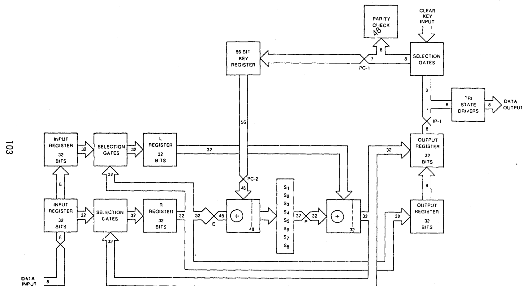
COMPLETE UNIT BLOCK DIAGRAM
