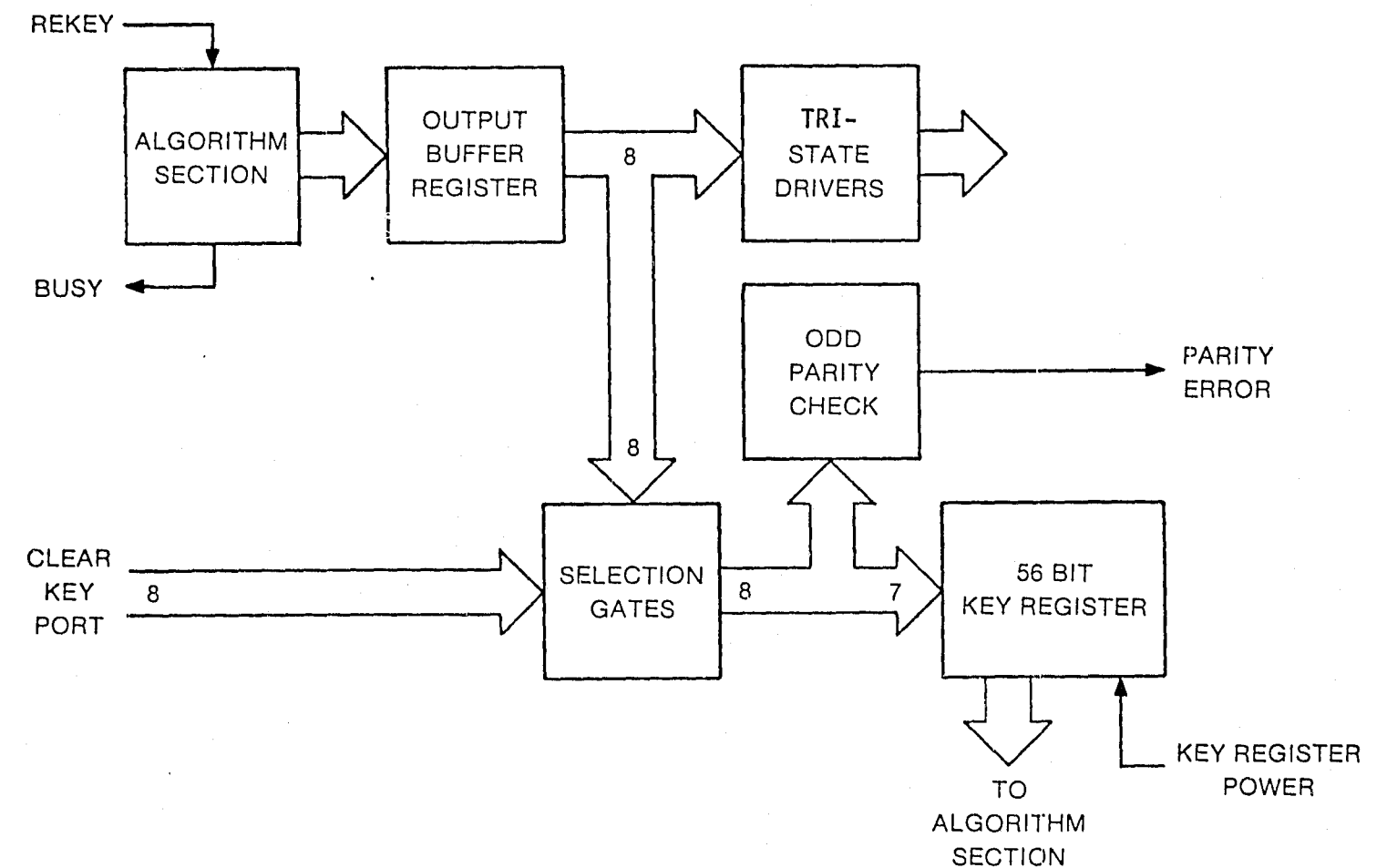
Figure 2. Key Path Block Diagram.
