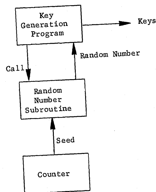
Figure 2 Key Generation
