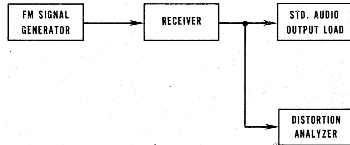
FIGURE 3. Block diagram for SINAD sensitivity measurement.
