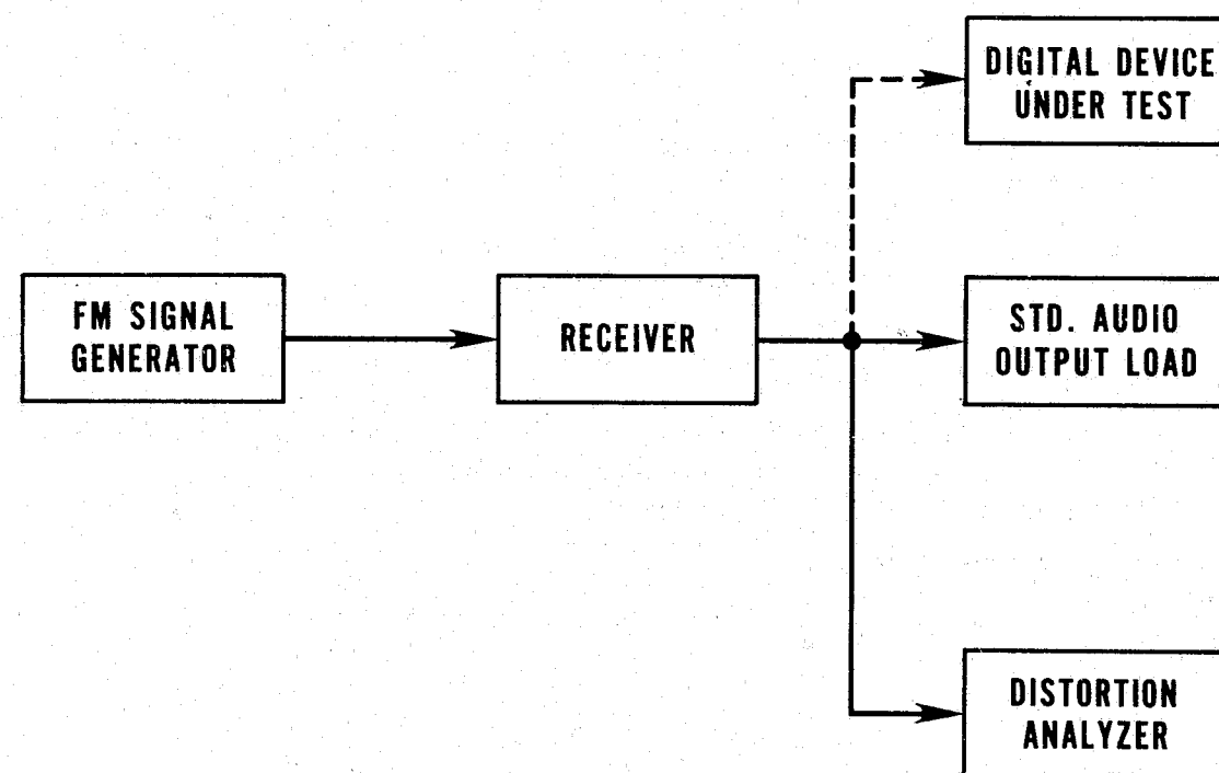
FIGURE 8. Block diagram for audio distortion loading measurement.
