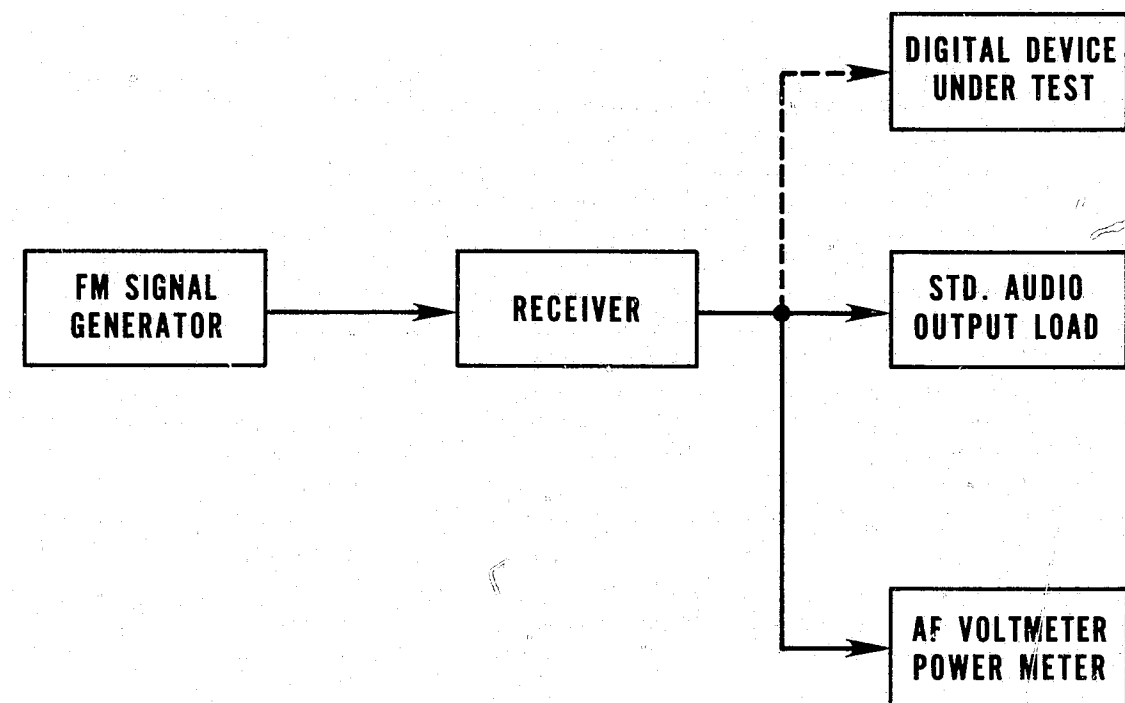
FIGURE 7. Block diagram for audio output power loading measurement.
