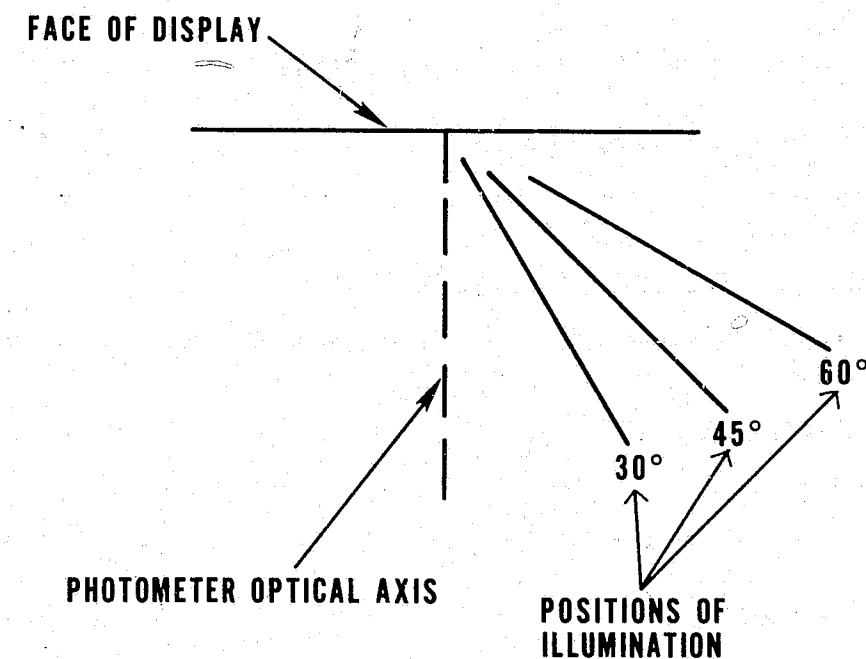
FIGURE 9. Block diagram for display readability measurement.
