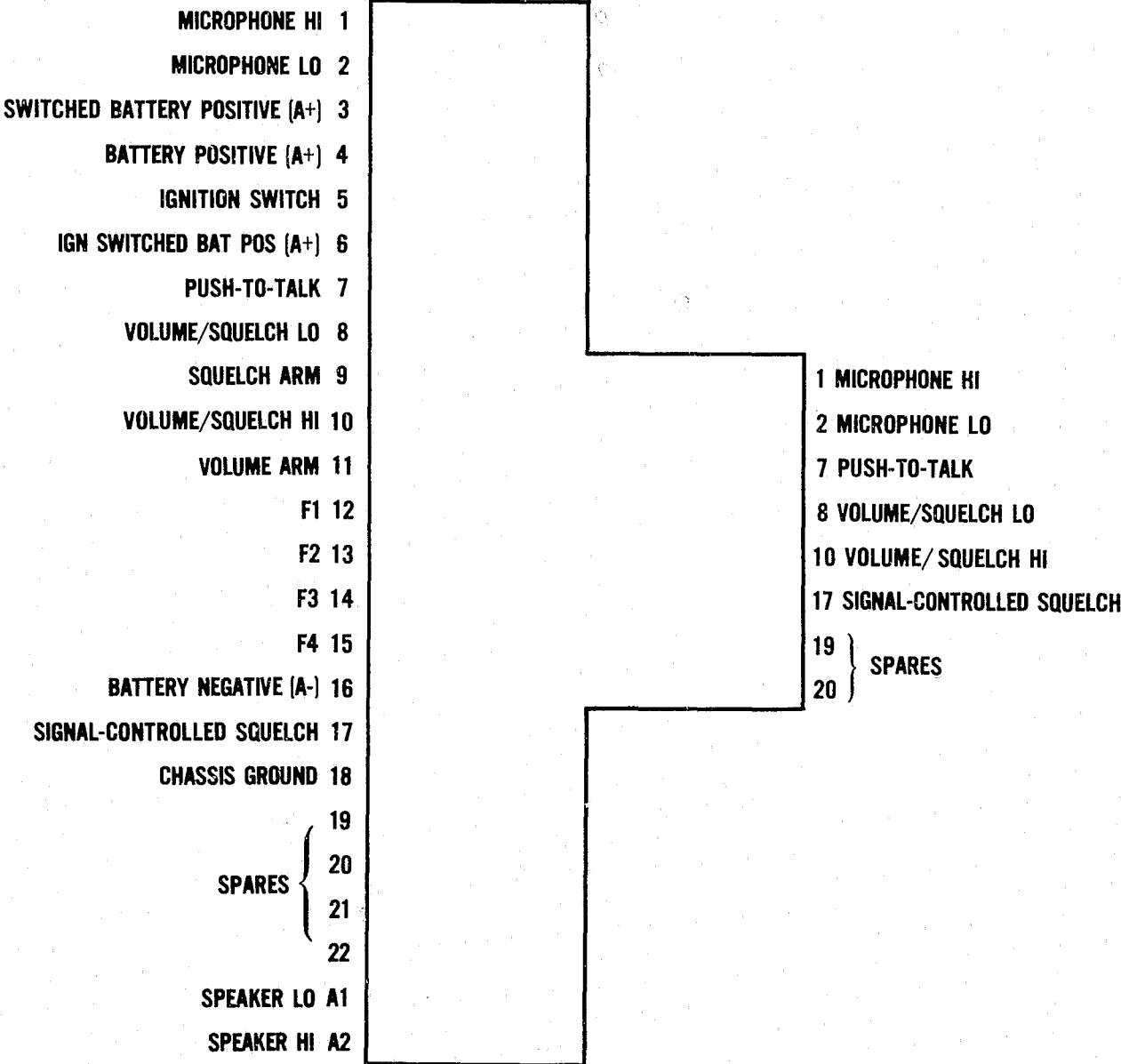
FIGURE 1. Tee connector.
