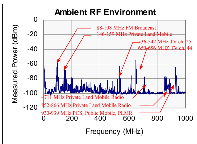
Figure 13. Ambient urban RF noise environment. Note the signal levels received from other radio services.
