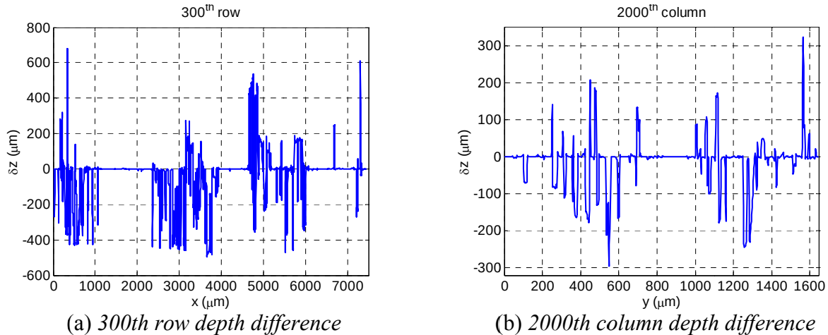
(a) 300th row depth difference (b) 2000th column depth difference Figure 6: The cross section of the difference between the raw data and the final data.
