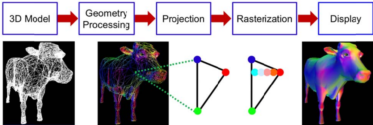
Figure 20: Computer graphics rendering pipeline (CGRP)
