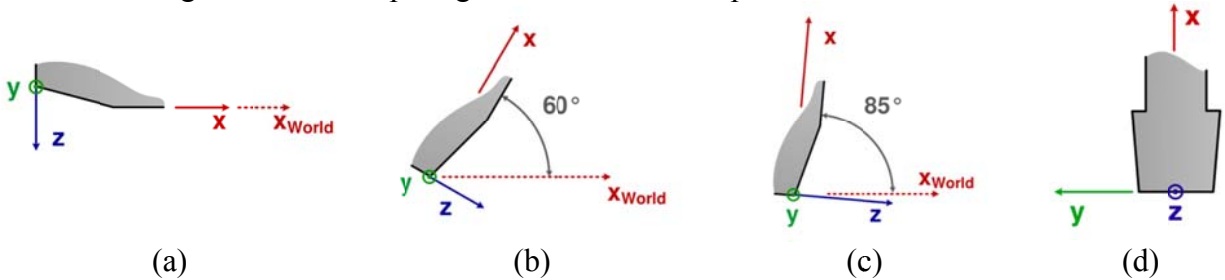
Figure 16: Tip coordinate system. (a-c) View of tip side. (d) View looking at the flat side of the screwdriver
