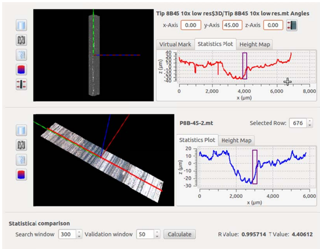
Figure 32: A known-match comparison between Tip 8B at 45 degrees and Plate 8B-45.
