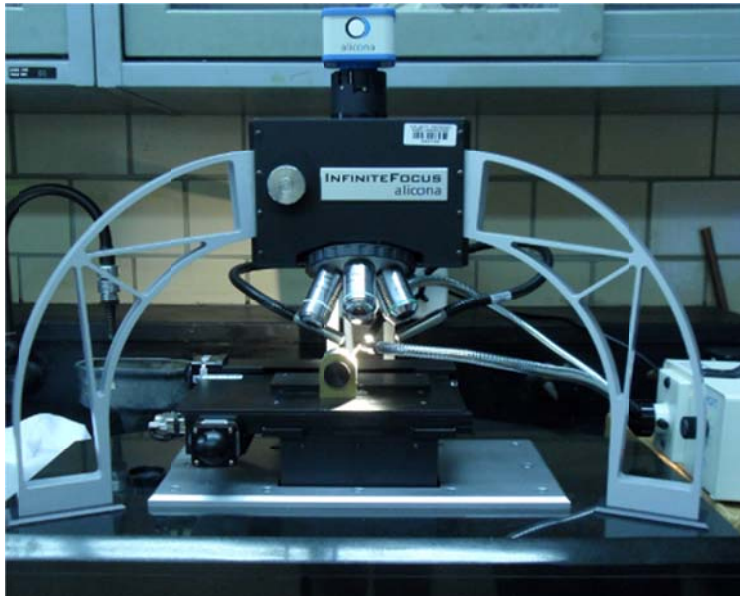
Figure 1 : Photo of the Alicona Infinite Focus Microscope (IFM)
