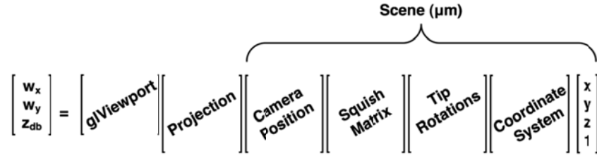
Figure 26: Mathematical model of the graphics pipeline for this research
