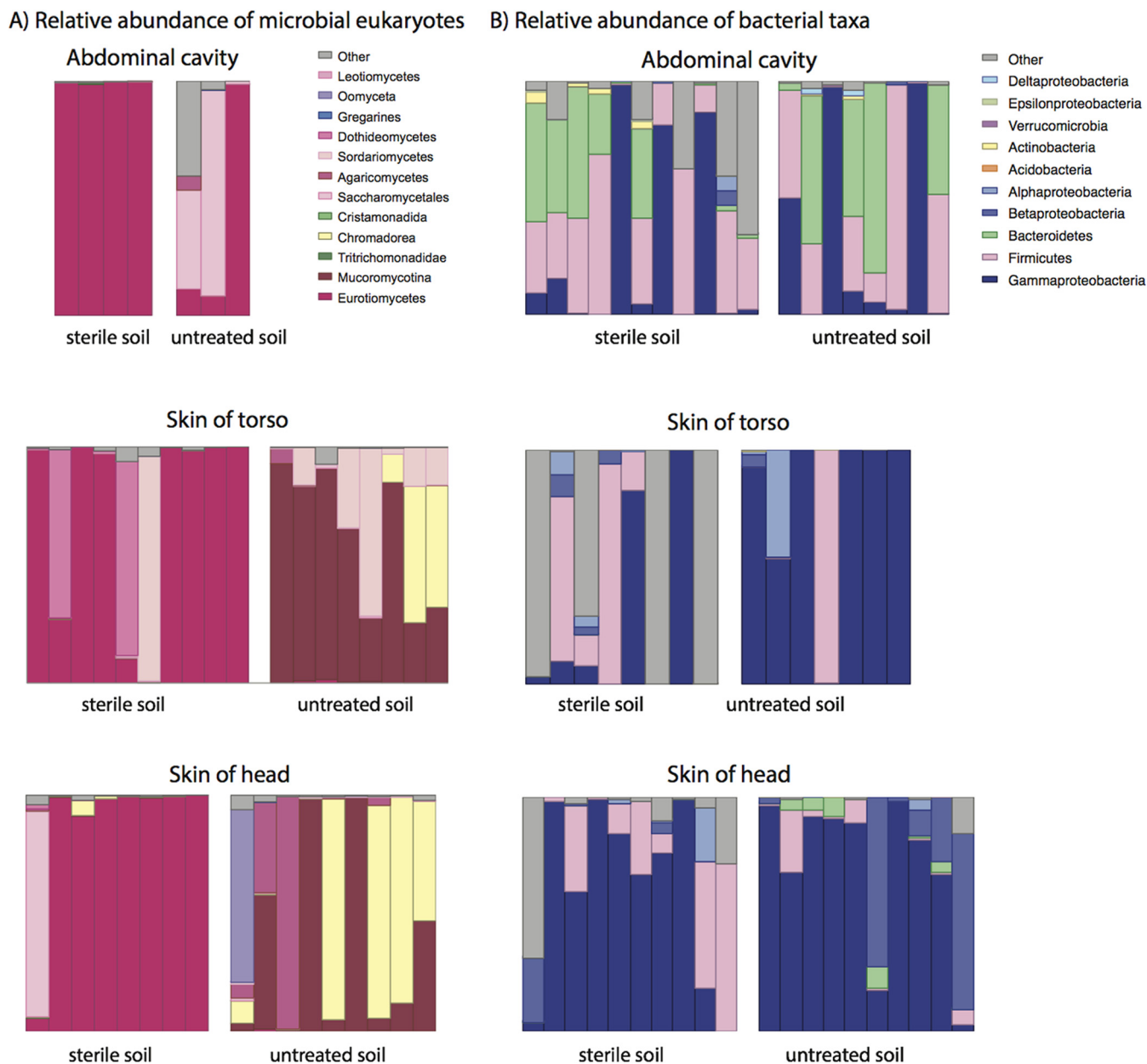
FIG 4 (A) Relative abundance of microbial eukaryotic taxa is shown at the highest level of taxonomic resolution for each sample site and each treatment (sterile versus untreated soil substrate). Each stacked bar shows the relative abundance of eukaryotes or bacteria in a single sample. Taxa are shaded by phylum: Fungi , red/pink; Excavata , green; Nematoda , yellow; Alveolata , blue; Stramenopiles , purple. Other low-abundance taxa are represented as gray. (B) Relative abundance of host-associated, late-stage decomposition bacterial communities with taxa abundance shown at the phylum level. Each bar in the figure represents the relative abundance of a given taxa for a single sample.
