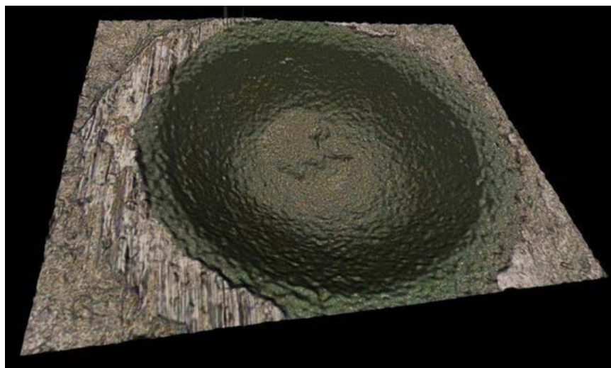
Figure 3. Firing pin impression on cartridge case measured with focus variation. Overlay of reflectance and topography images.
