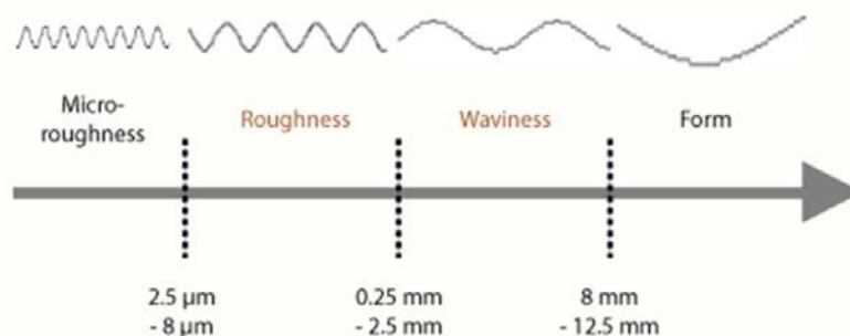
Figure 4. Four components of surface texture 12
