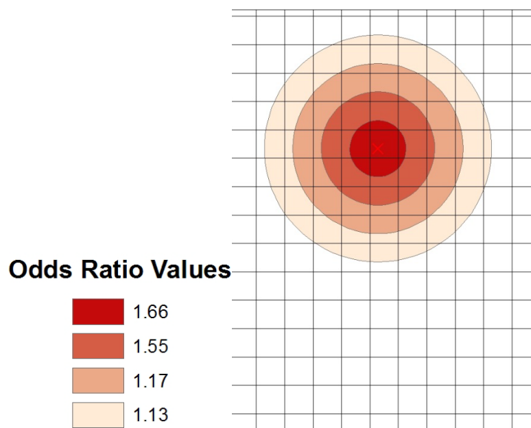
Figure 5: Risk of near repeat crime decreasing with distance
