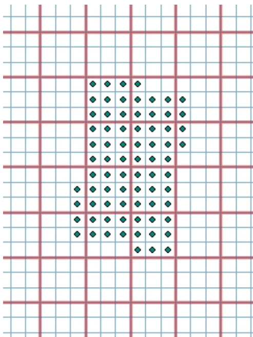
Figure 4: Aggregation to coarse cells
