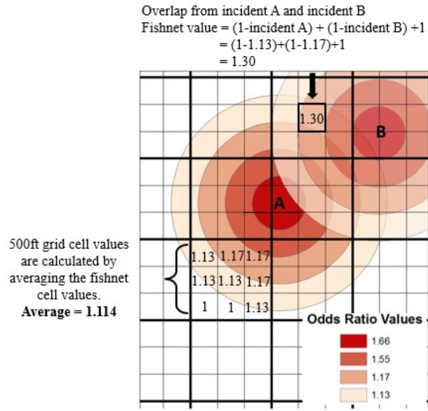
Figure 1 Boost Calculation. “A” and “B” represent separate crime incidents in the 28 day period.
