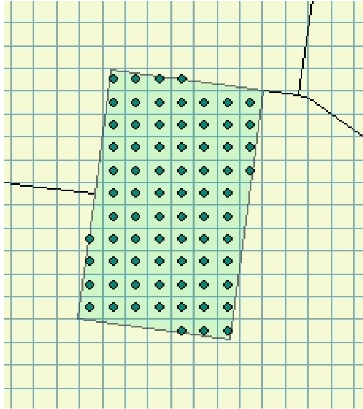
Figure 2 Fishnet centroid locations.
