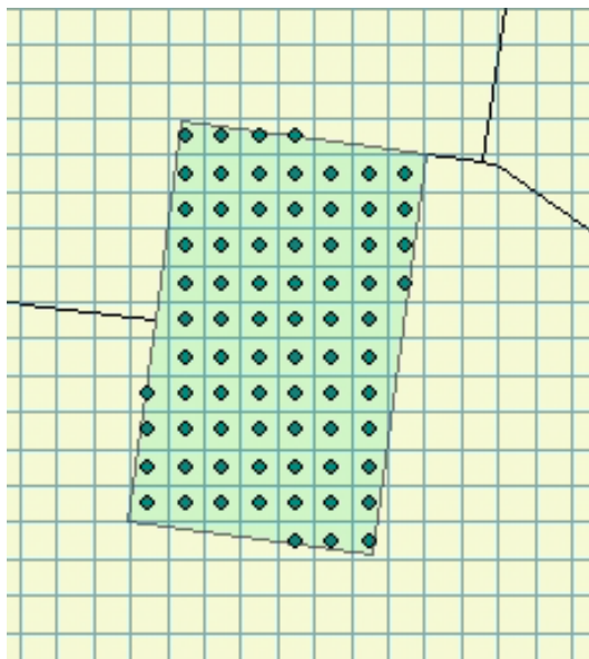
Figure 3: Cells assigned a value of 1.129
