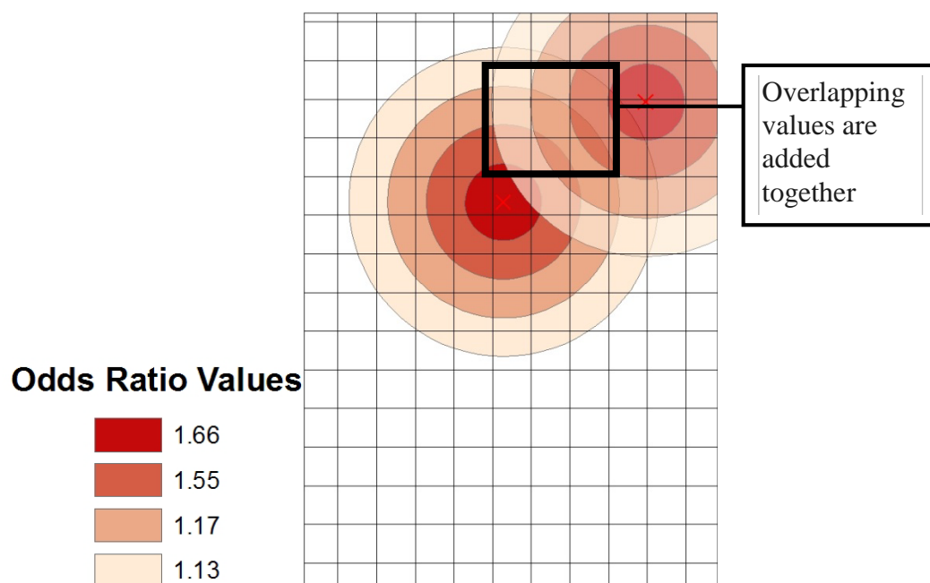
Figure 6: Assigning risk to overlapping areas
