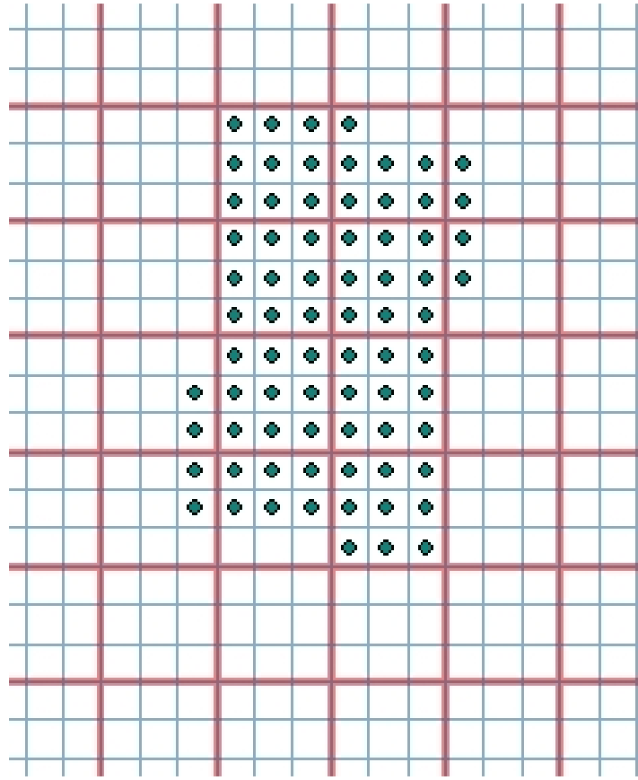
Figure 3 Centroids with respect to 500 foot grid cells.
