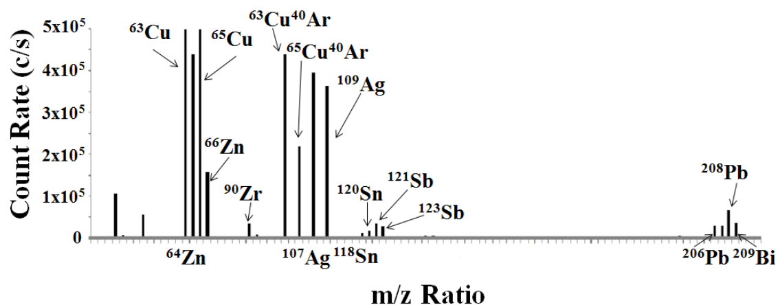
FIG. 2—Average mass spectrum for two copper strands ablated with the fs laser and measured by ICP-MS. Peaks with significant count rates (c/s) were labeled, m/z ratios were measured from 7 Li to 238 U. Peaks below m/z 63 were not labeled due to polyatomic interferences.
