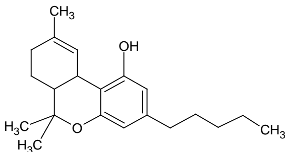
Fig. 1.1. Chemical diagram (decarboxylated form) of THC
